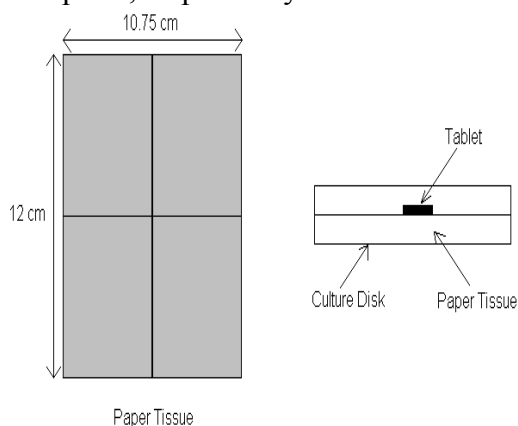
FIG.1. It shows schematization measurement of tablet wetting time and water absorption ratio
