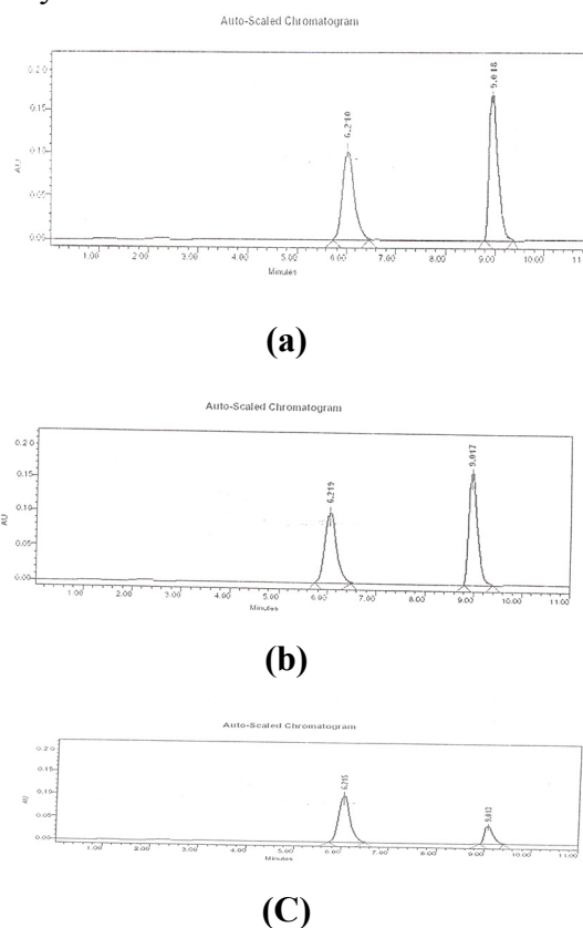
FIG. 2. It shows chromatograph obtained for (a) a sample solution (combination of Omeprazole and Domperidone) (b) dissolution of Omeprazole (c) dissolution of Domperidone.
